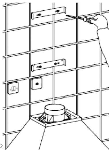
Mount chimney brackets
